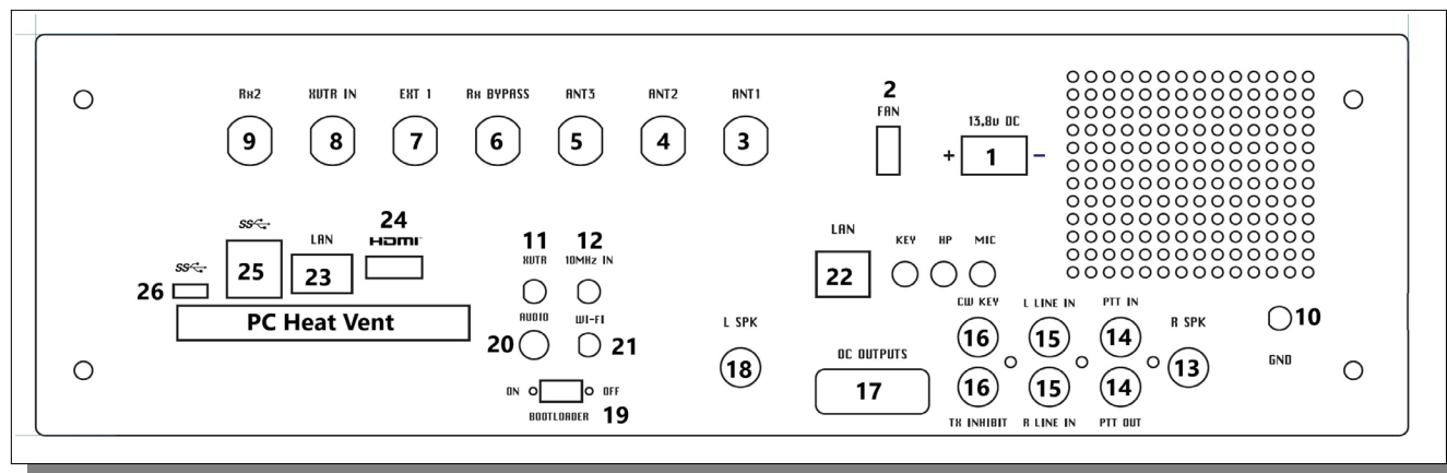
ANAN-7000DLE MKII back panel details
